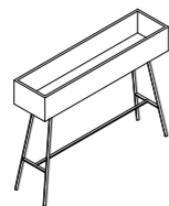
Planter (High) H925 W1200 D300
