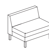
One Seat Armless Sofa, Config with Booth W900 D690 H700
