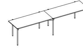
Single Bench L1050-1650 H745 D525-825
